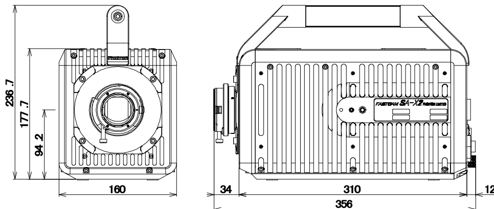
All dimension are given in millimeter
