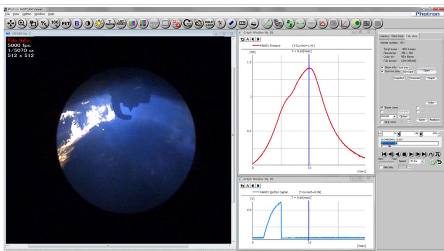
Photron FASTCAM Viewer image display together with synchronised data acquisition measurement
